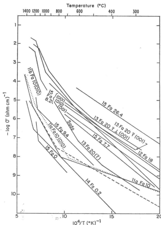
Fig. 3. Conductivity of olivine single crystals as determined by this and other studies. Composition is indicated above the line. Question mark means that the composition of olivine was not reported by the author. Numbers in parentheses give the direction in which \sigma measurement was made. First number above the line refers to one of the following investigators: 11a, Hughes [1953]; 11b, Hughes [1955]; 12, Mizutani and Kanamori [1967]; 13, Noritomi [1961]; 14, Shankland [1969].
